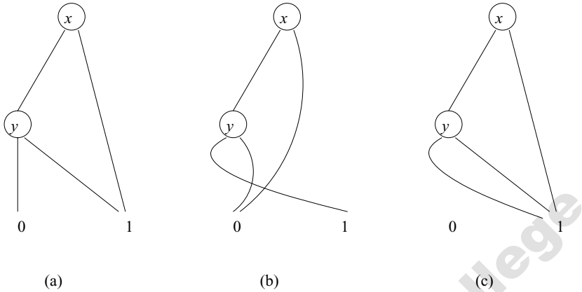
Figure 12.33: Constructing the BDD for a logical OR
