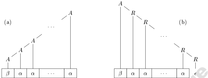
Figure 2.20: Left- and right-recursive ways of generating a string
