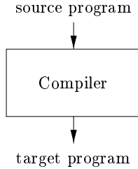
Figure 1.1: A compiler
