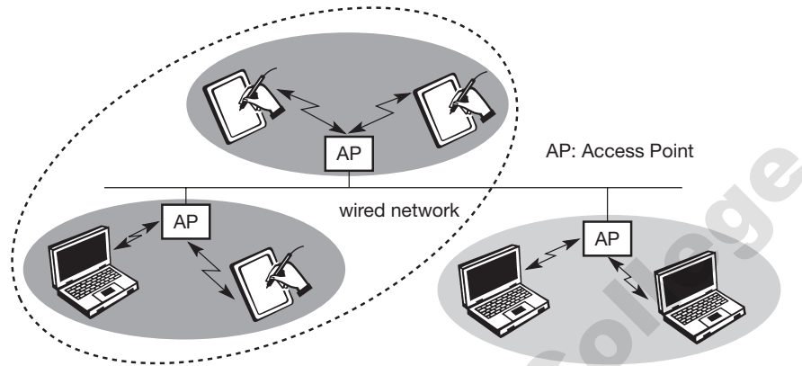
Figure 7.1 Example of three infrastructure-based wireless networks
