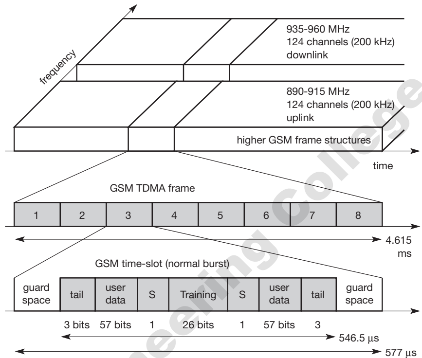
Figure 4.5 GSM TDMA frame, slots, and bursts
