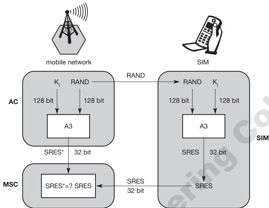
Figure 4.14 Subscriber authentication
