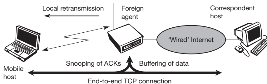
Figure 9.3 Snooping TCP as a transparent TCP extension
