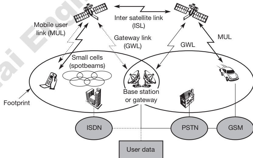
Figure 5.1 Typical satellite system for global mobile telecommunications
