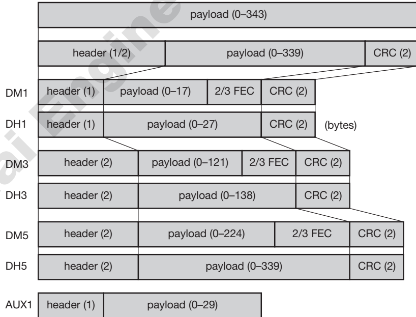
Figure 7.48 ACL payload types
