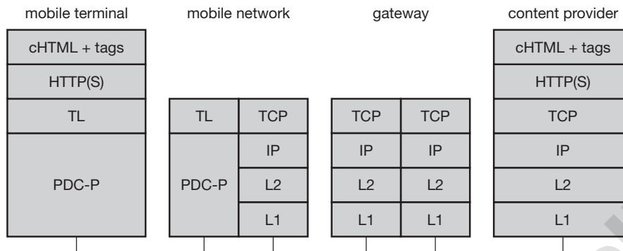
Figure 10.34 i-mode protocol stacks for Japan
