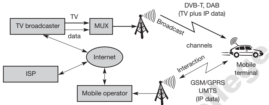
Figure 6.10 Mobile Internet services using IP over GSM/GPRS or UMTS as interaction channel for DAB or DVB
