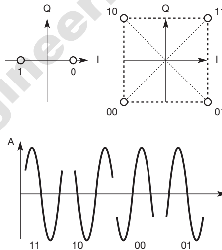
Figure 2.27 BPSK and QPSK in the phase domain
