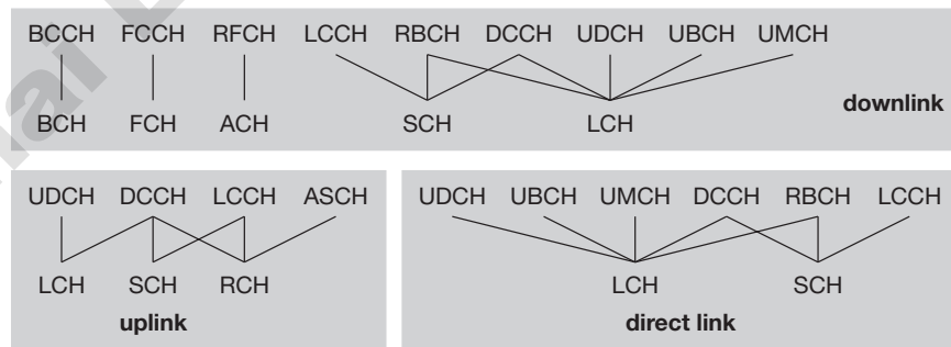
Figure 7.38 Mapping of logical and transport channels
