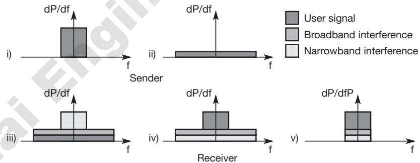
Figure 2.32 Spread spectrum: spreading and despreading
