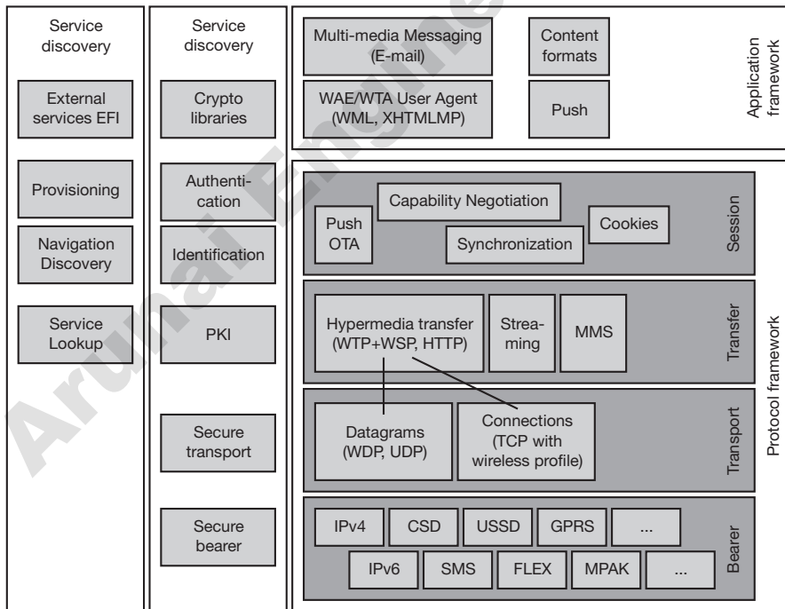
Figure 10.37 WAP 2.0 architecture
