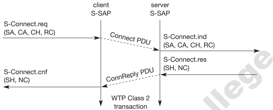
Figure 10.20 WSP/B session establishment
