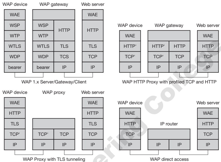
Figure 10.38 Example protocol stacks according to WAP 2.0
